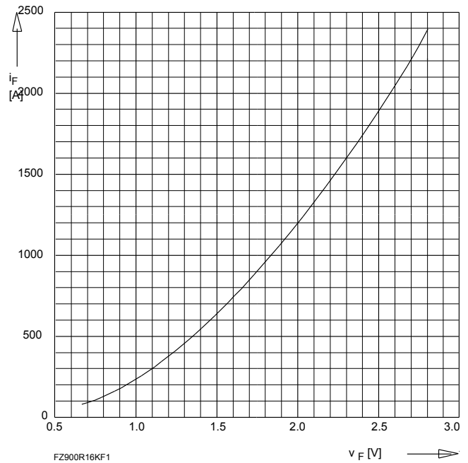
Bild/Fig. 6 Forward characteristic of the inverse diode (typical) characteristic of the inverse diode (typical) ..... t_{vj} = 25^{\circ}C — t_{vj} = 125^{\circ}C
